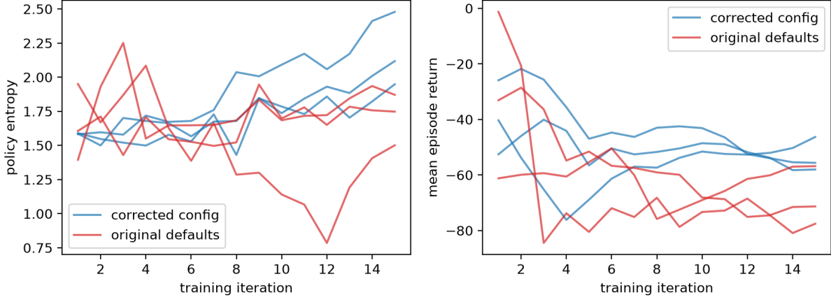
Figure 1: Policy entropy (left) and mean episode return per iteration (right) for the six runs, three per configuration. The original defaults (red) do not collapse; one run dips to 0.79 at iteration 12 and recovers.
