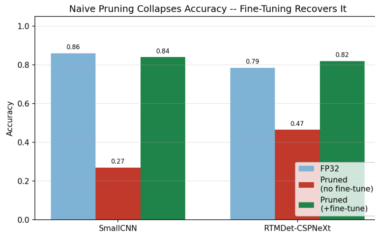
Figure 5.6. Naive pruning collapse vs. fine-tune recovery.
