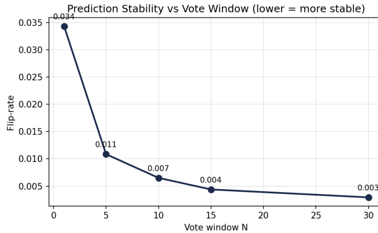
Figure 5.4. Flip-rate vs vote window size.
