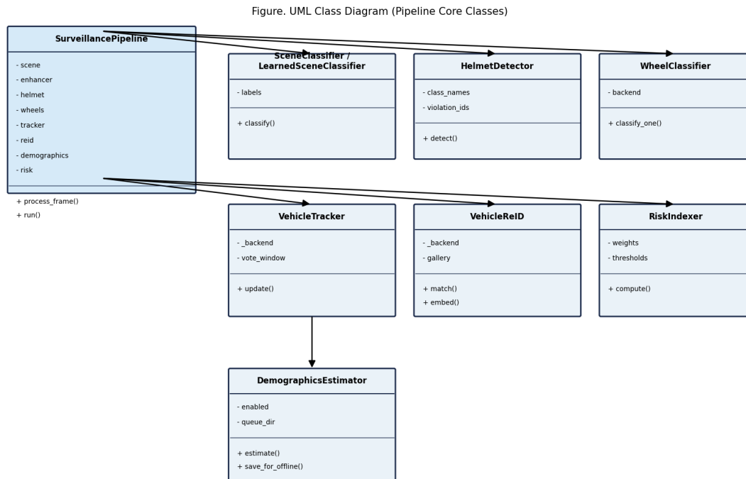
Figure 4.4. UML class diagram of the pipeline's core classes, with real attribute and method names taken directly from the source modules.
