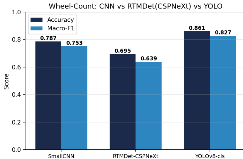
Figure 5.2. Accuracy and macro-F1, leak-free split.
