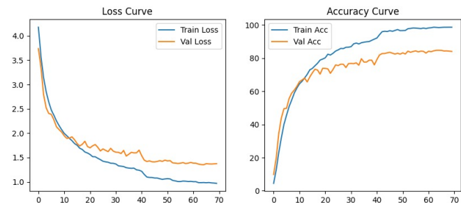
Fig. 8. Accuracy Curve(Resnet).
