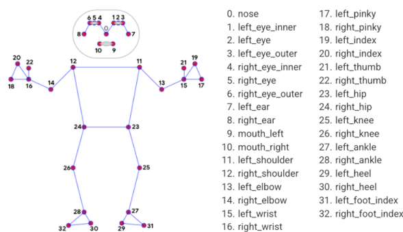
Fig. 3. BlazePose Model - Topology as depicted in the original paper.
