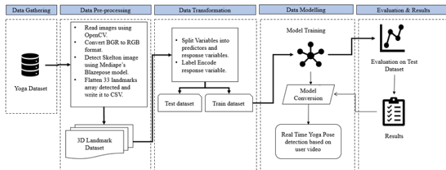
Fig. 2. Methodology - Real-time Yoga Pose Detection pipeline.
