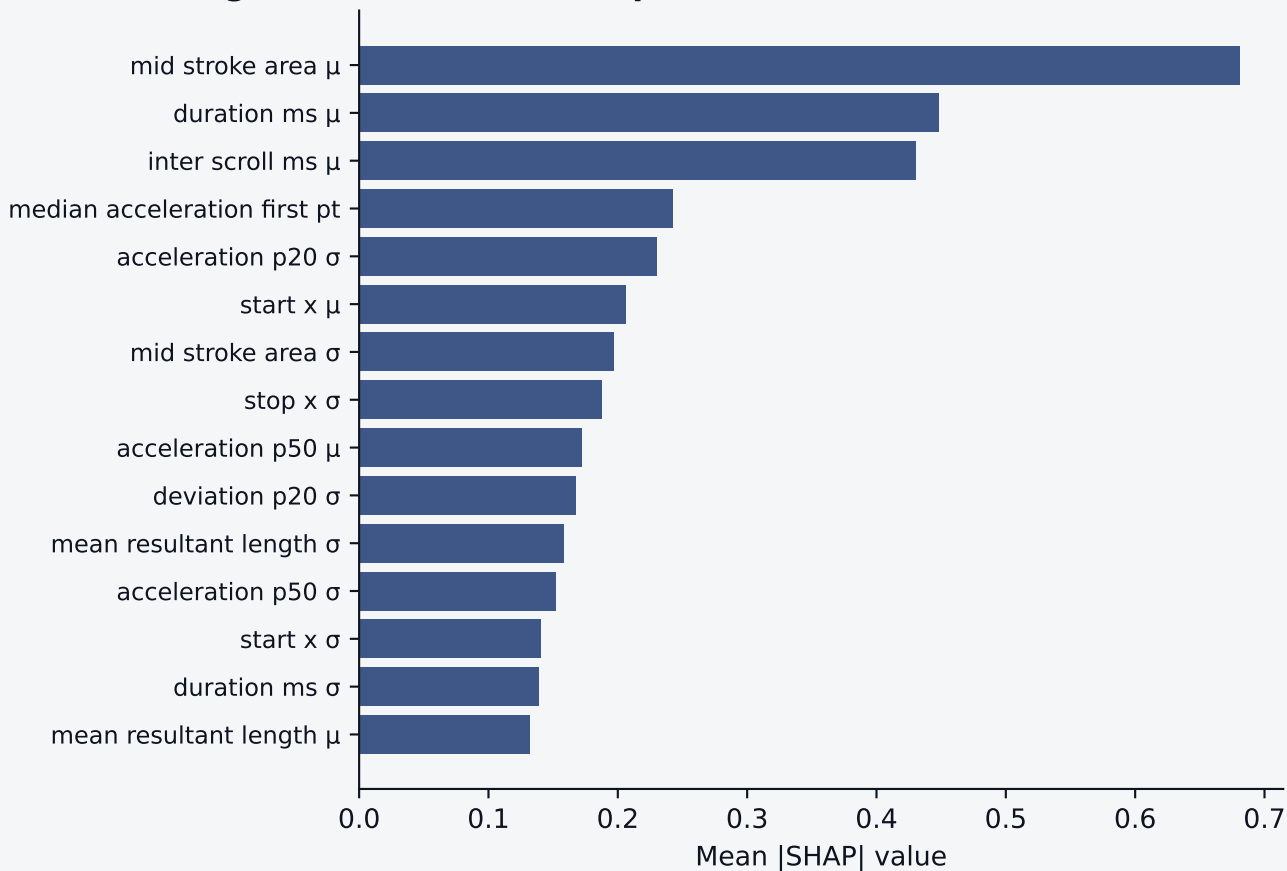
fig-08 SHAP Feature Importance (XGBoost, HMOG sit->walk, top 15)
