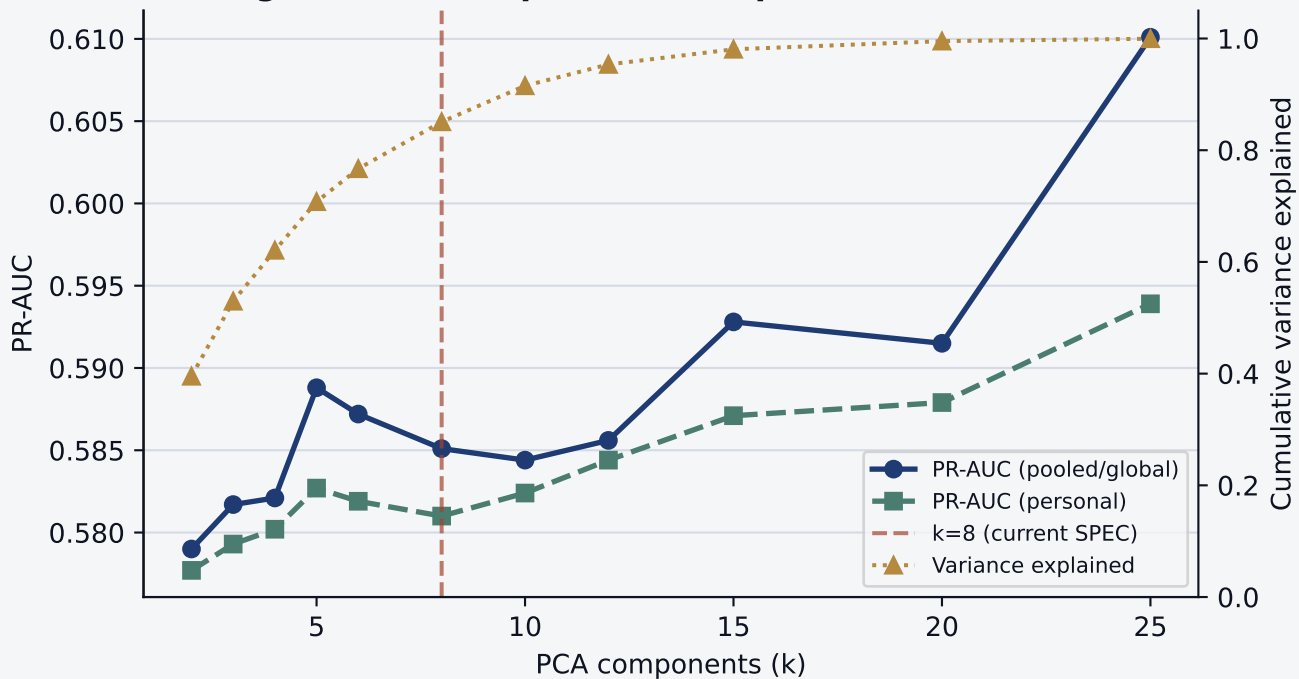
fig-09 PCA Component Sweep (HMOG sit->walk)
