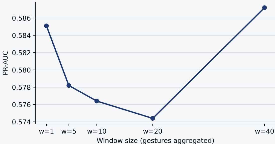
fig-10 Session Aggregation (PCA Reconstruction, HMOG sit->walk)
