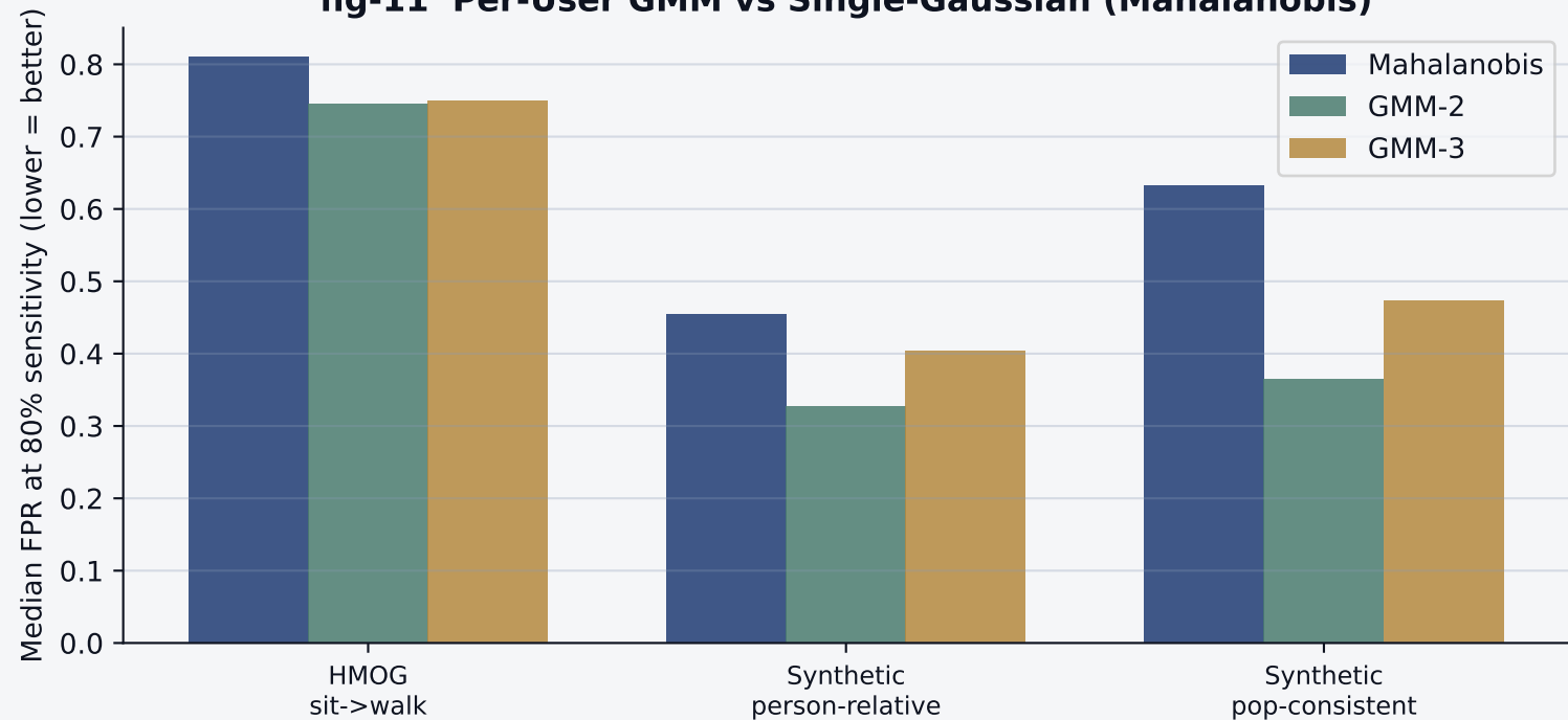
fig-11 Per-User GMM vs Single-Gaussian (Mahalanobis)
