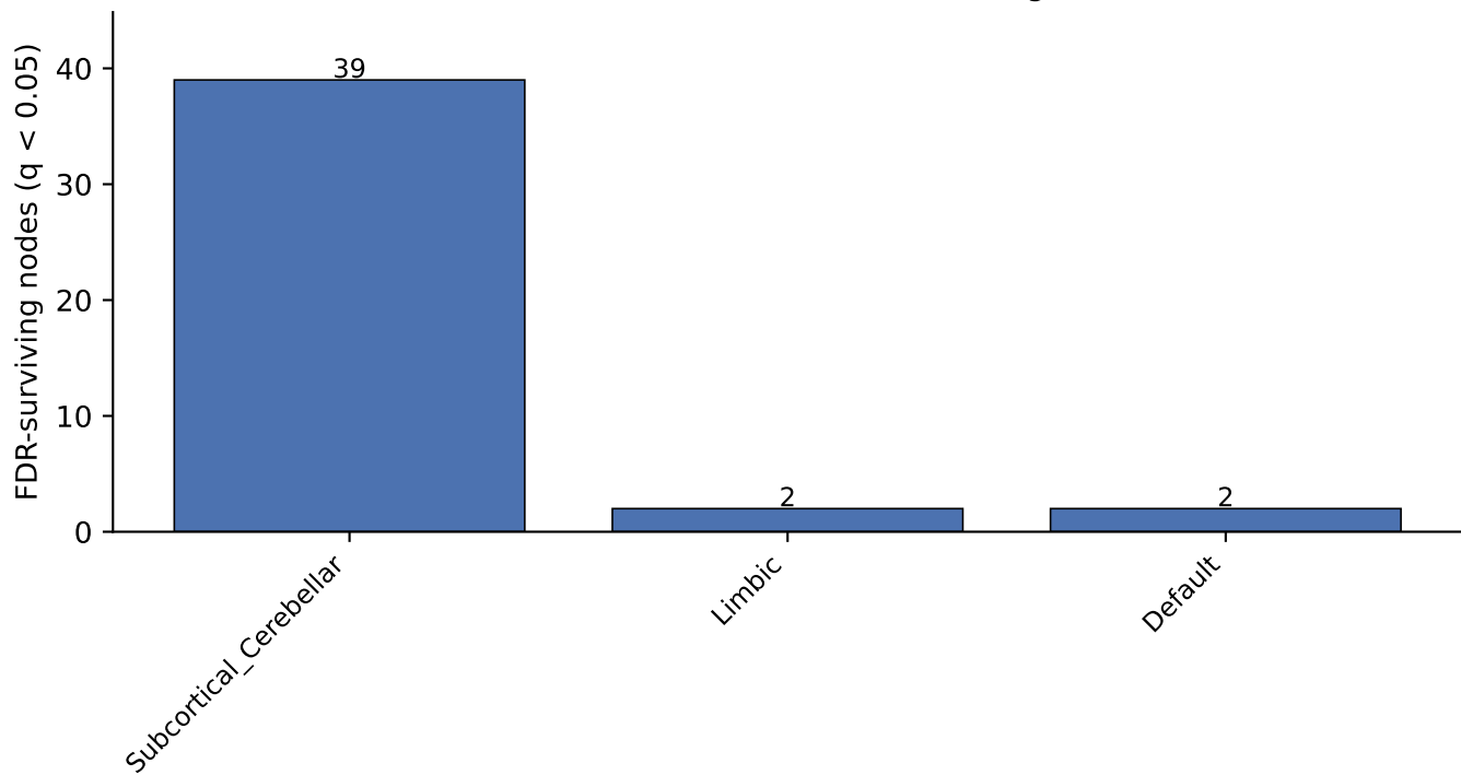
Anatomical distribution of the 43 FDR-surviving nodes (4S456)
