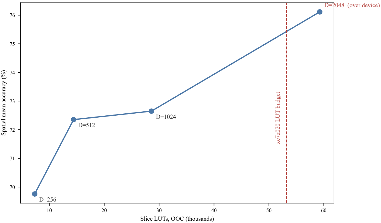
Hook A — accuracy vs area Pareto (CNT_W=6, unpruned)
