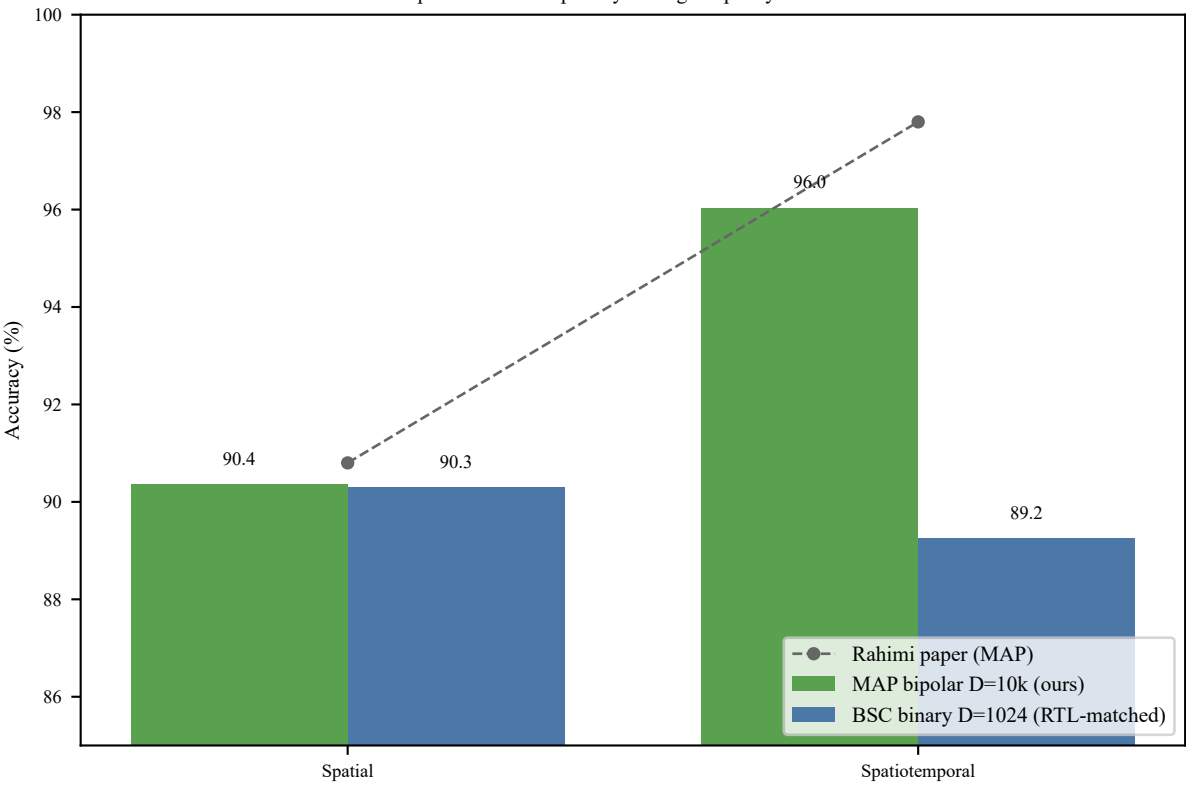
Temporal context helps only the high-capacity MAP model
