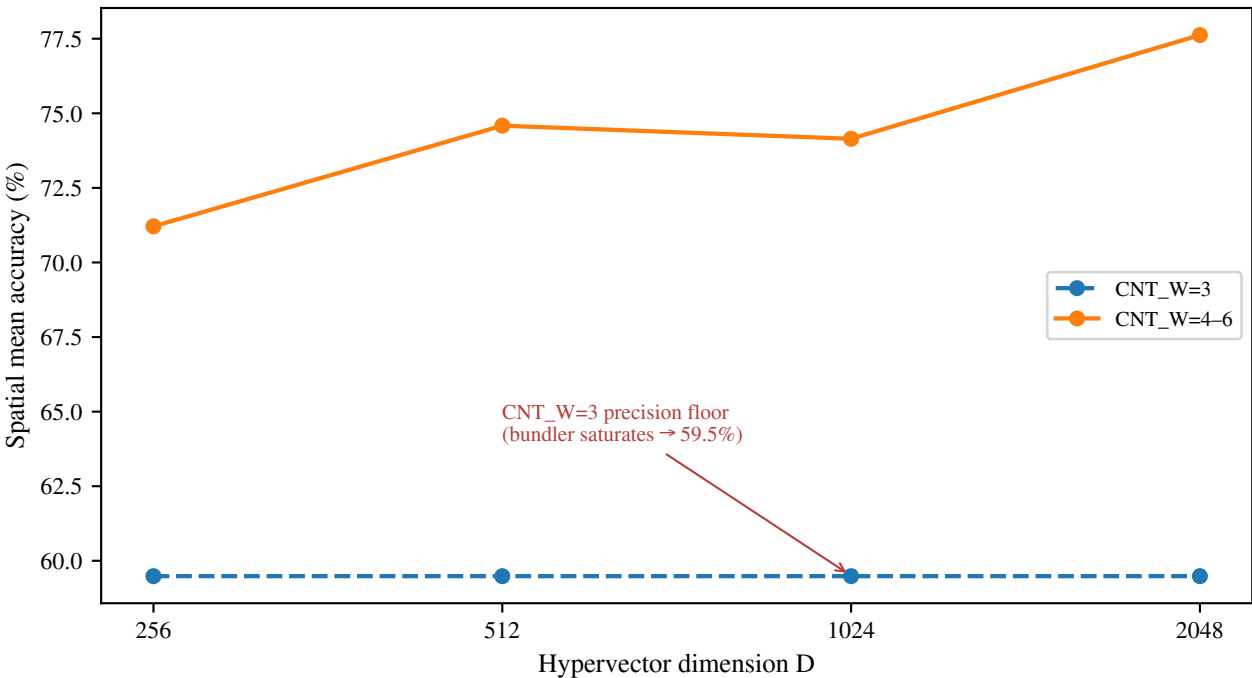
Hook A — accuracy vs D and bundle-counter width
