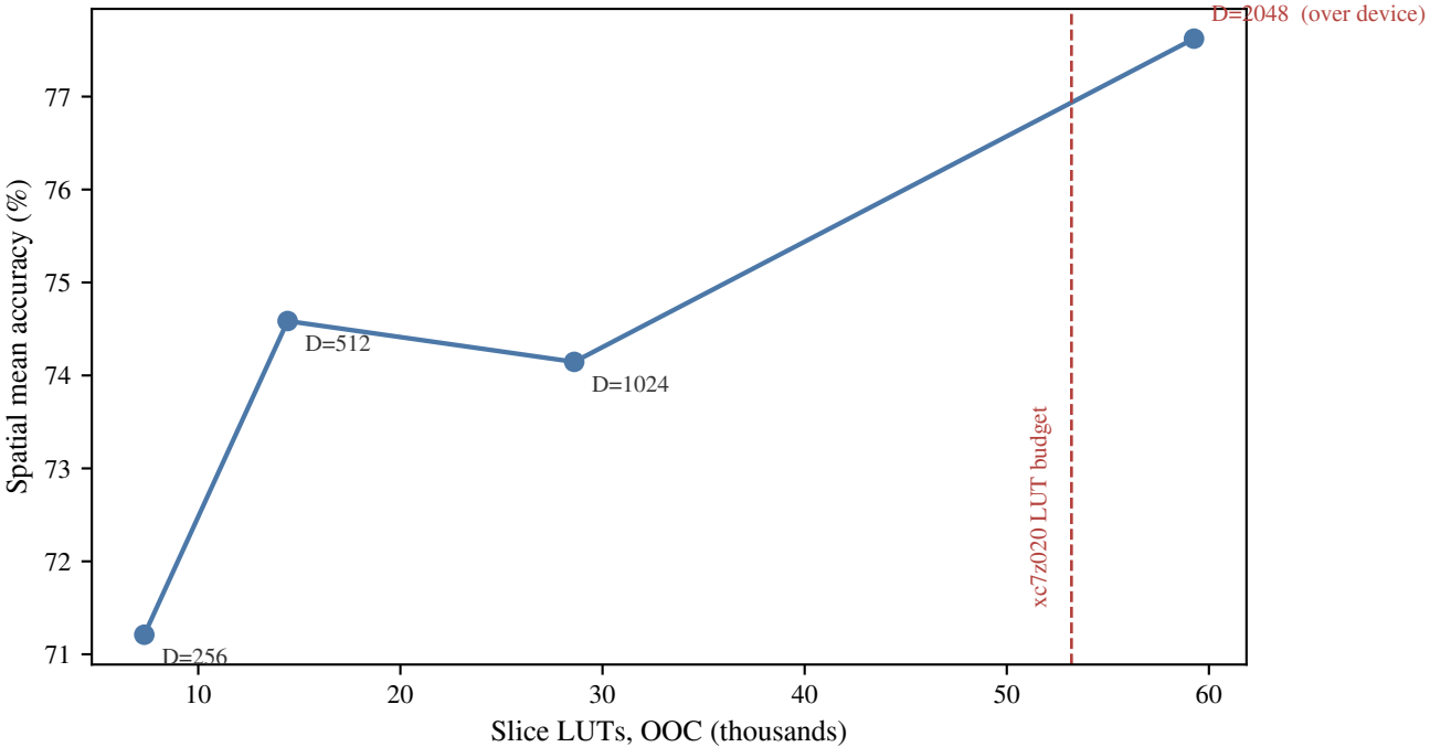
Hook A — accuracy vs area Pareto (CNT_W=6, unpruned)
