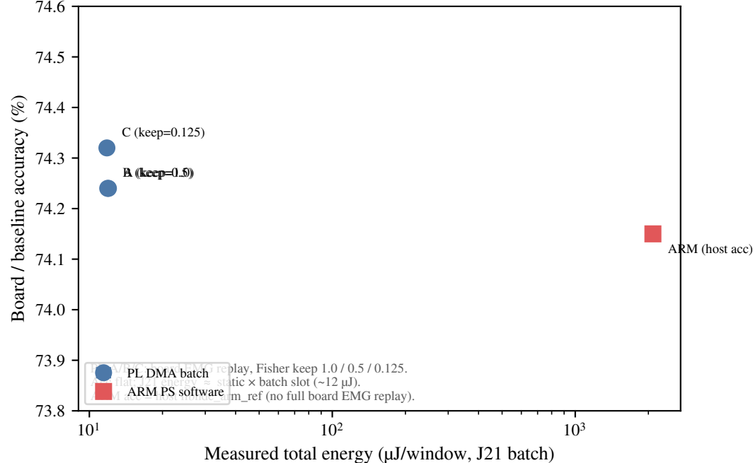
(b) Measured energy — flat PL, ARM ~175× (static-dominated PL)
