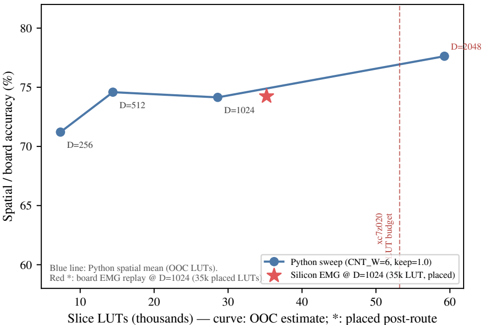
(a) Accuracy vs area — Python OOC sweep + placed silicon
