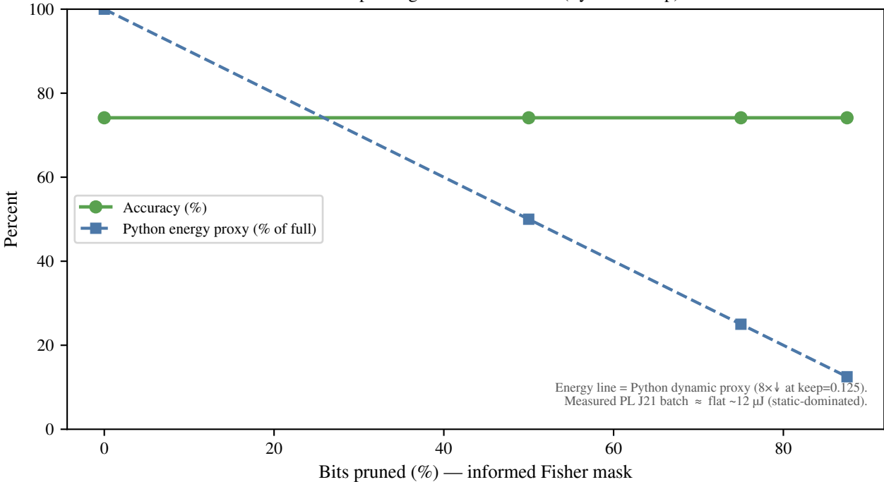
Hook A — pruning is free @ D=1024 (Python sweep)
