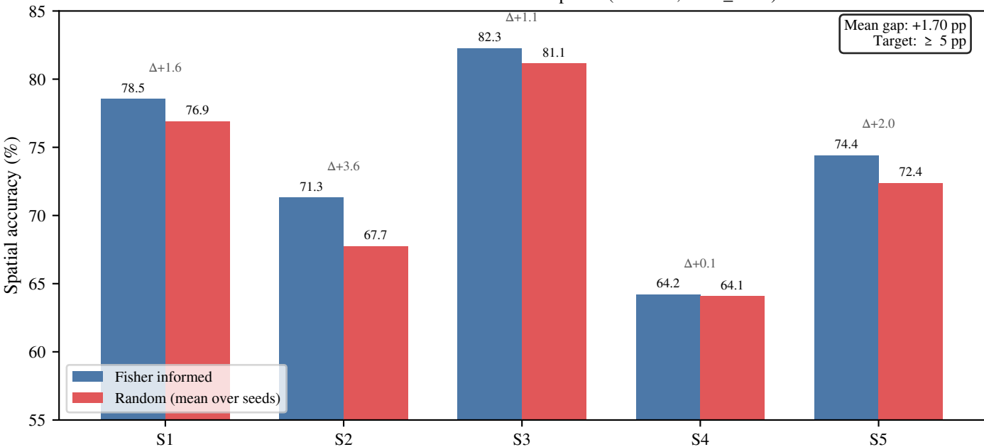
Twist 1 — informed vs random @ keep=0.5 (D=1024, CNT_W=6)
