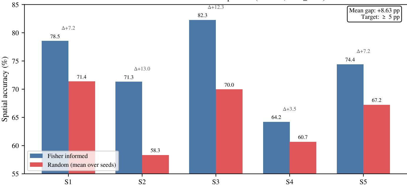
Twist 1 — informed vs random @ keep=0.125 (D=1024, CNT_W=6)
