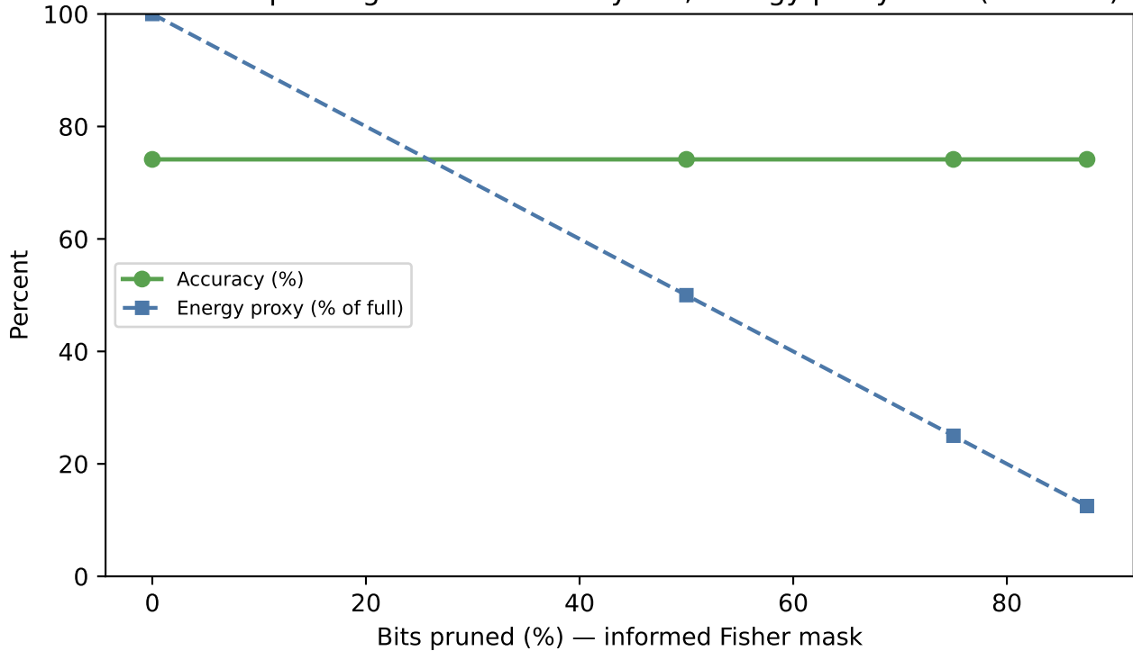
Hook A — pruning is free: accuracy flat, energy proxy 8\times\downarrow (D=1024)
