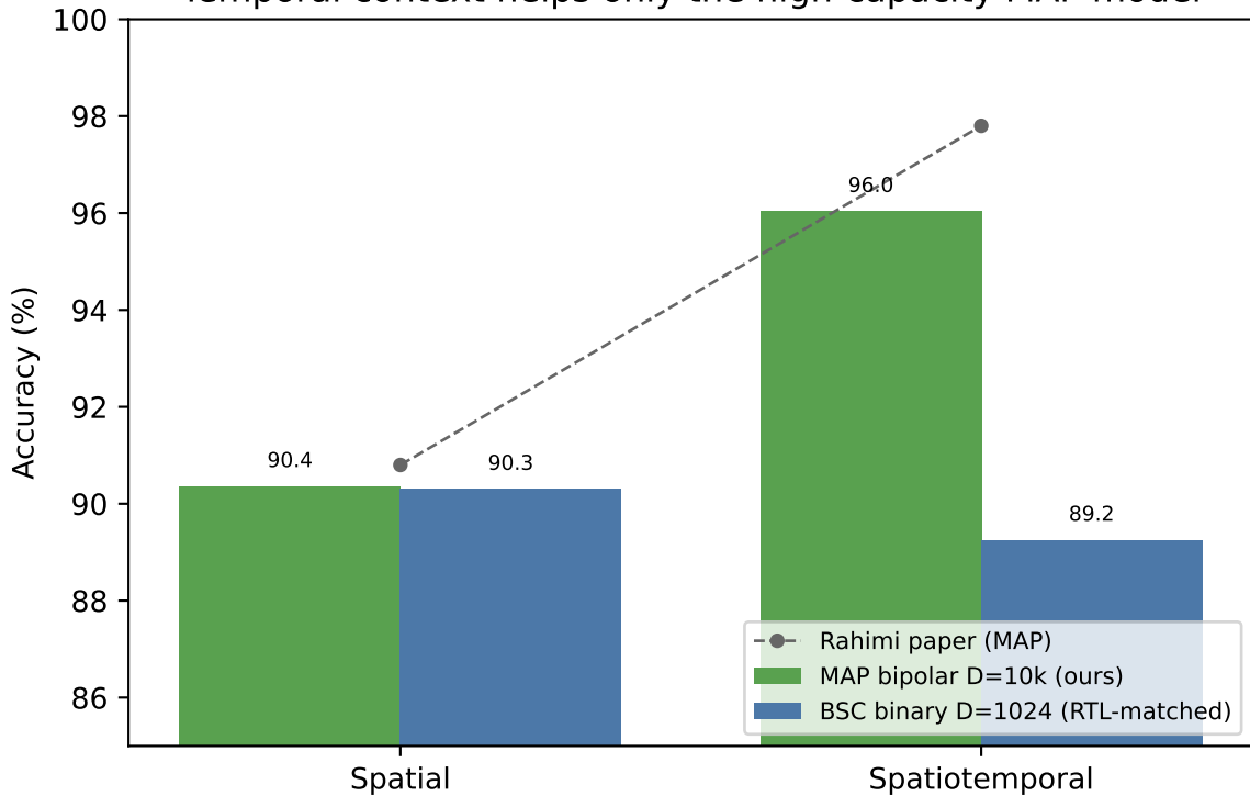
Temporal context helps only the high-capacity MAP model
