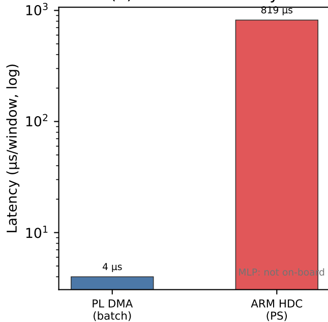
(b) On-board latency
