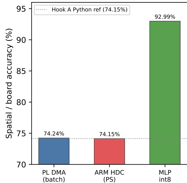
(a) Accuracy
