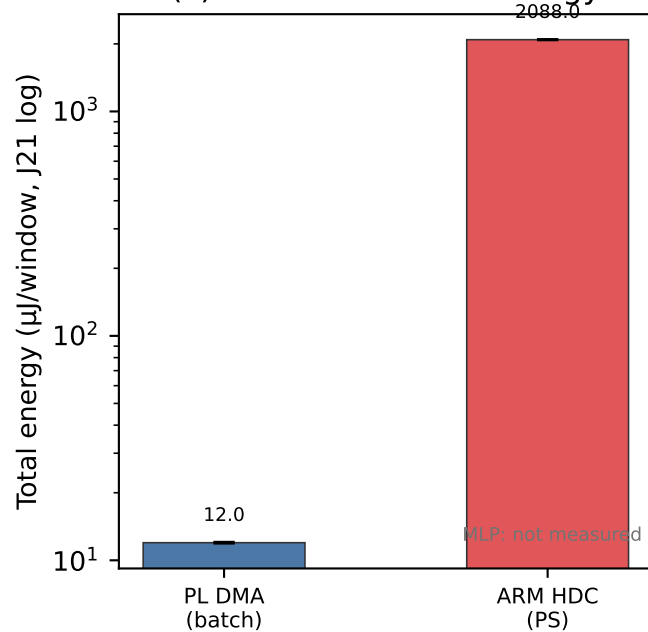
(c) Measured batch energy
