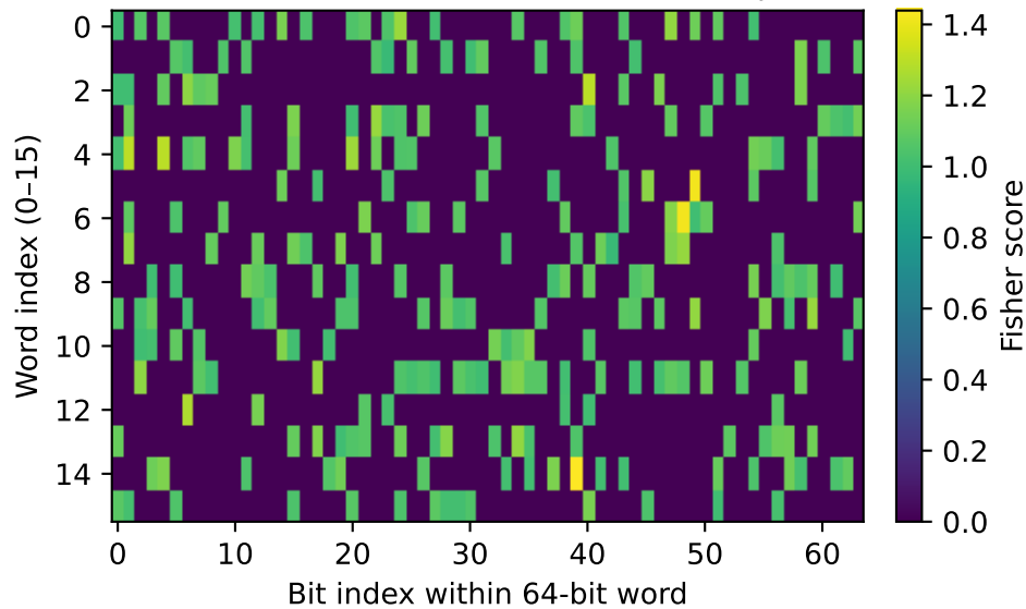
(c) Informed mask @ keep=0.5
