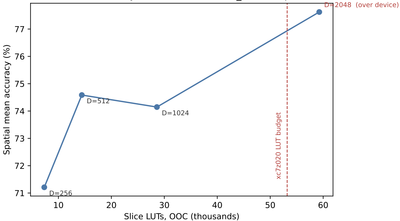
Hook A — accuracy vs area Pareto (CNT_W=6, unpruned)
