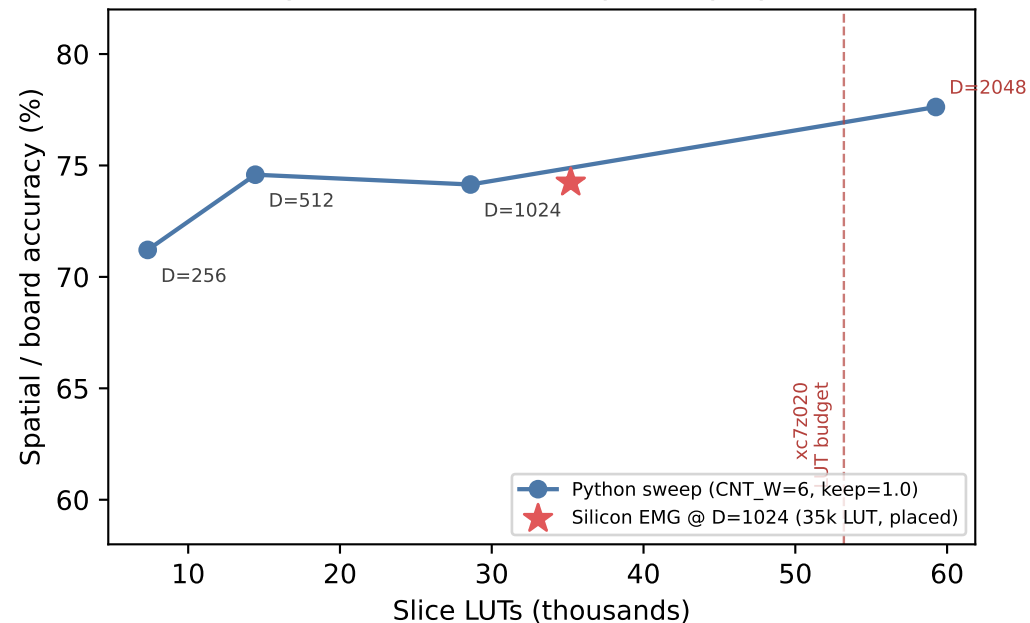
(a) Accuracy vs area — D sweep + deployed bitstream
