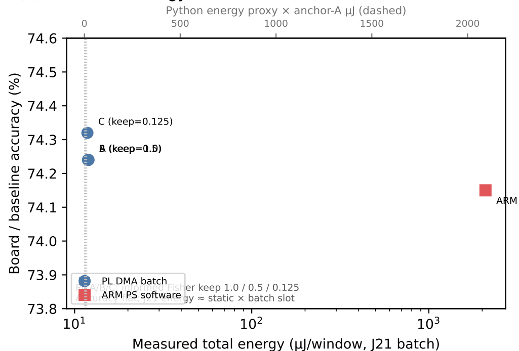
(b) Measured energy — flat PL, ARM ~175× (static-dominated PL)
