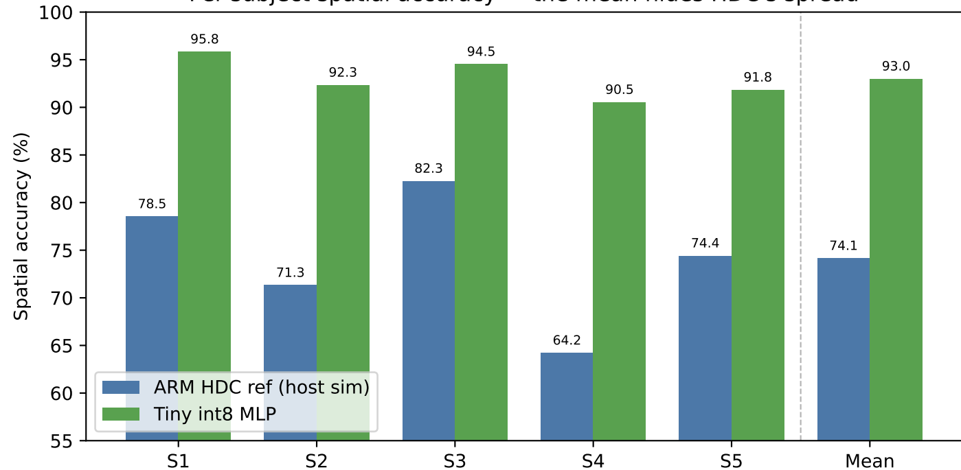
Per-subject spatial accuracy — the mean hides HDC's spread
