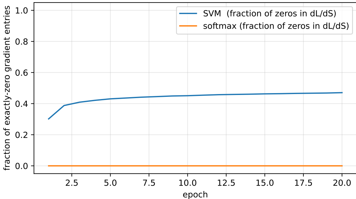
Score-gradient sparsity vs. epoch
