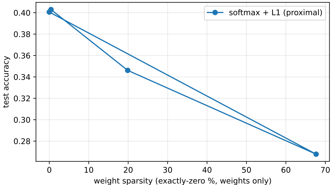
Accuracy vs. L1 sparsity
