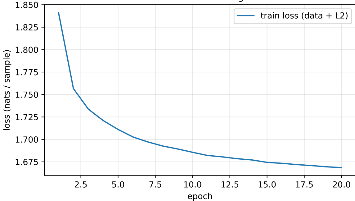
Best softmax: training loss
