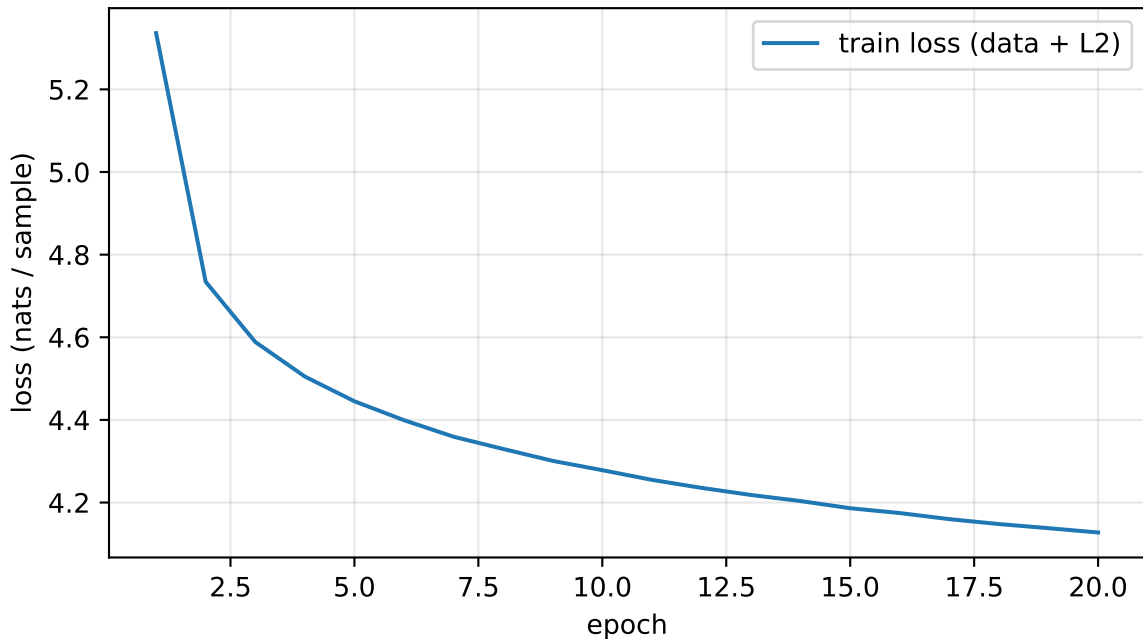
Best multiclass SVM: training loss
