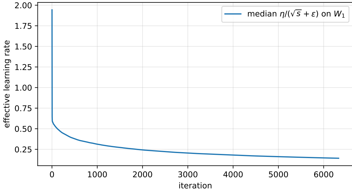
AdaGrad effective step size on first-layer weights
