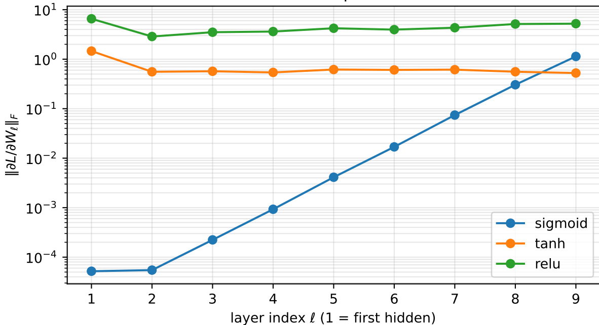
Gradient scale vs. depth at initialization
