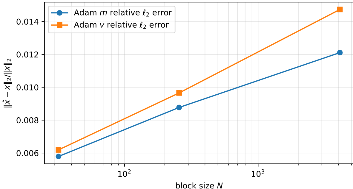
Block-wise INT8 quantization error vs. block size
