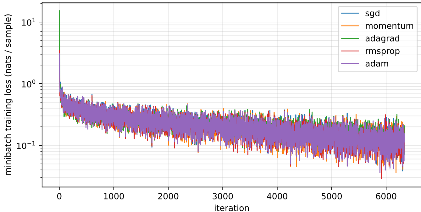
Training loss of the five best optimizer runs
