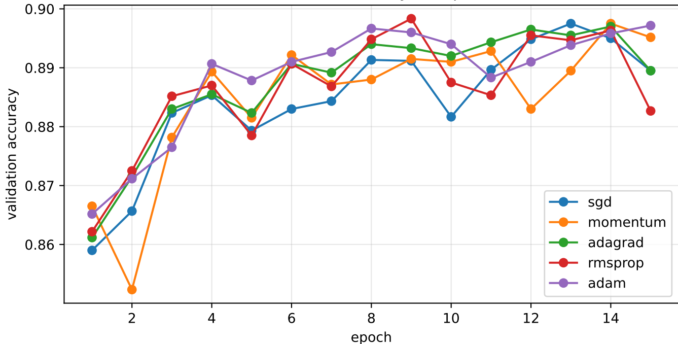
Validation accuracy vs. epoch
