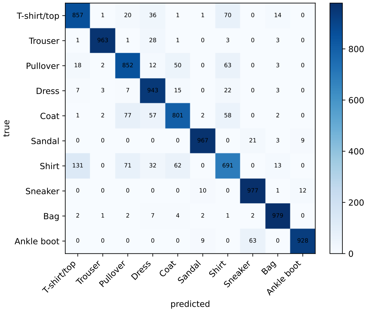
Fashion-MNIST confusion matrix
