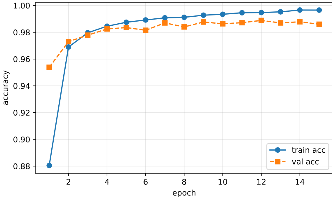
LeNet-5 baseline: accuracy vs epoch
