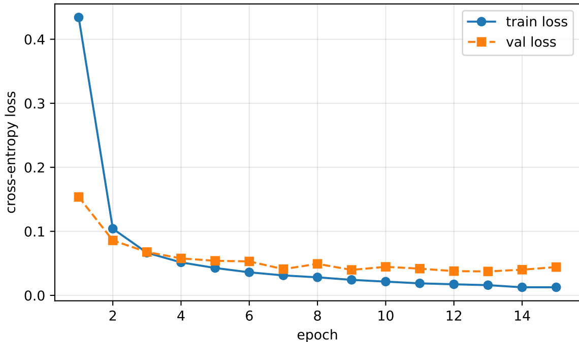
LeNet-5 baseline: loss vs epoch
