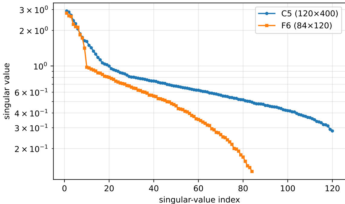
Singular-value spectra of C5 and F6 (log y)
