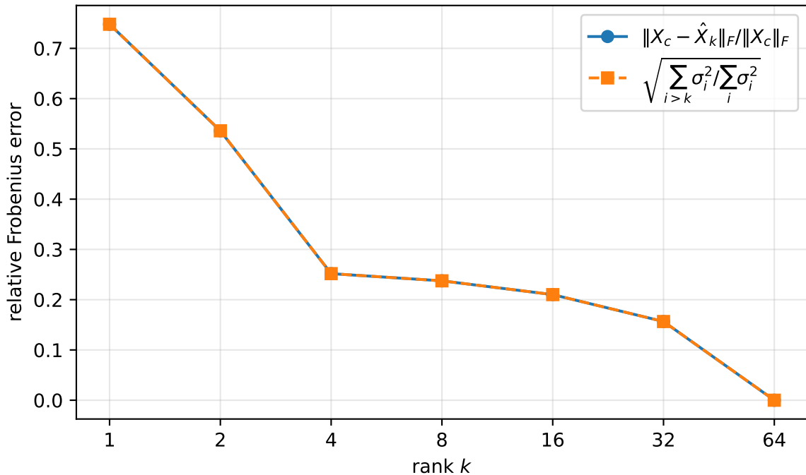
Reconstruction error vs. truncated-SVD bound
