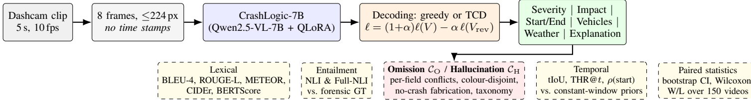
Fig. 2. CrashX systems and evaluation stack. CrashLogic-7B is a QLoRA adaptation of Qwen2.5-VL-7B trained to emit serialised forensic fields and a free-text Explanation; Temporal Contrastive Decoding (TCD) optionally contrasts its logits against a reversed-frame negative at decode time. Every output is scored for lexical overlap, entailment, separate omission and hallucination costs with a field-level decomposition, and temporal grounding against prior-only baselines, with all comparisons paired over the same 150 test videos.
