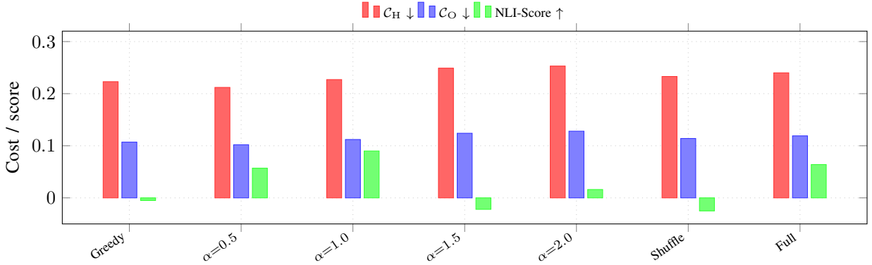
Fig. 3. Decoding ablation on CrashLogic-7B (Table XVII). Hallucination and omission costs are flat from greedy to \alpha=1.0 and rise significantly at \alpha\geq 1.5 ; NLI-Score peaks at \alpha=1.0 but its paired interval includes zero at every \alpha (Table III, Table V).
