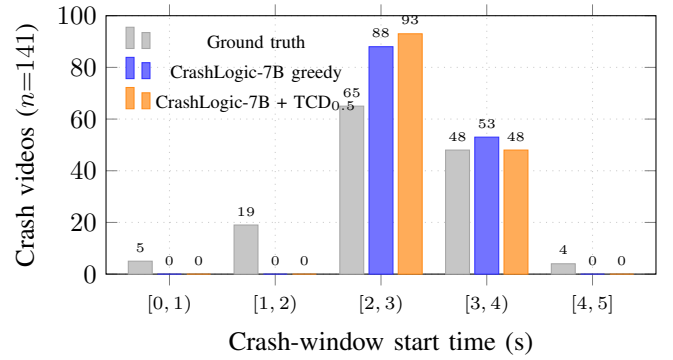
Fig. 1. The temporal prior. Ground-truth crash starts span the whole clip; the adapted model predicts only 2 s or 3 s, always with a 1-second window, matching the two most frequent training windows. Predicted and true starts are uncorrelated (Spearman \rho=0.009 greedy, 0.028 TCD), and a constant [3, 4] s window scores higher fIoU than either system (Table IV).
