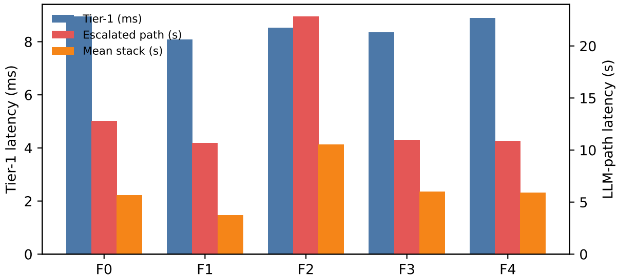
Latency: Tier-1 vs escalated LLM path
