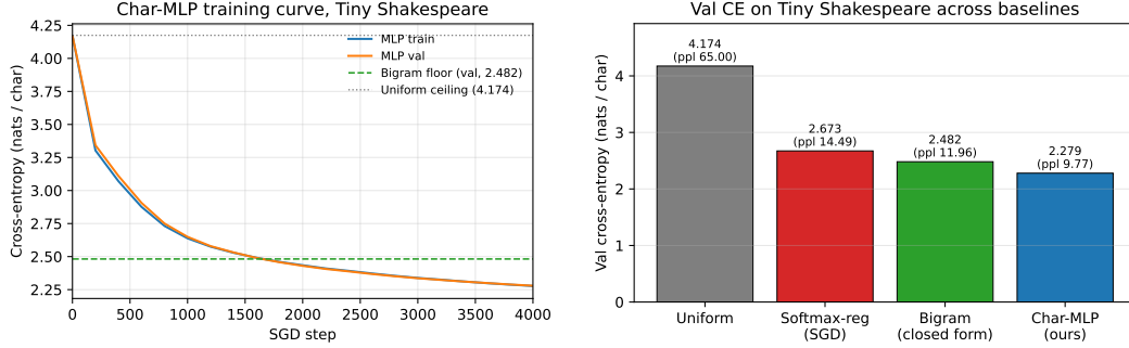
(a) MLP train+val CE vs. SGD step. Val crosses the bigram floor (dashed green) around step 1700. (b) Val CE across the four reference points. Lower is better.
