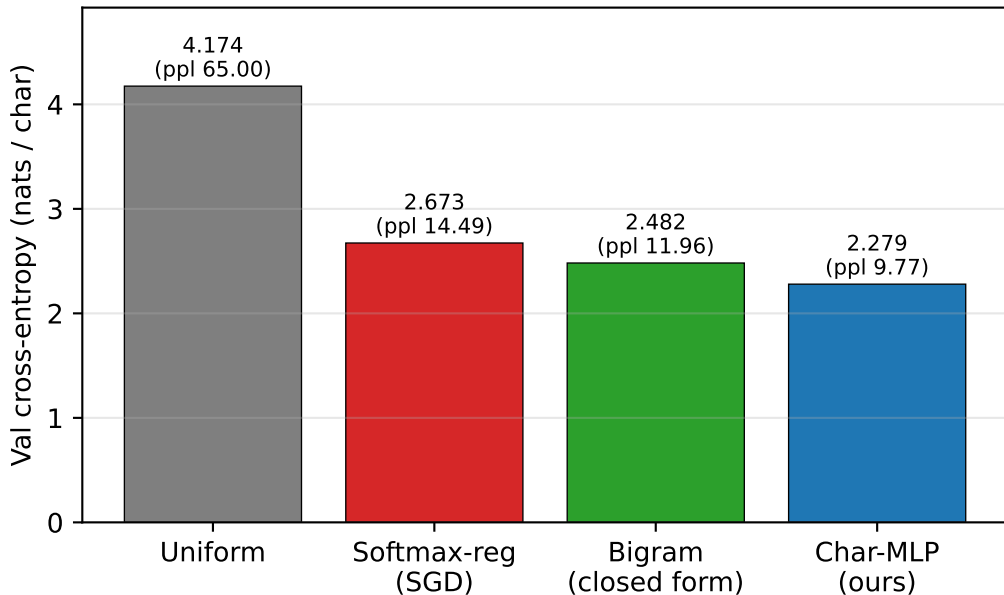
Val CE on Tiny Shakespeare across baselines
