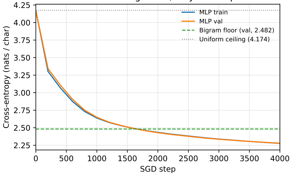
Char-MLP training curve, Tiny Shakespeare
