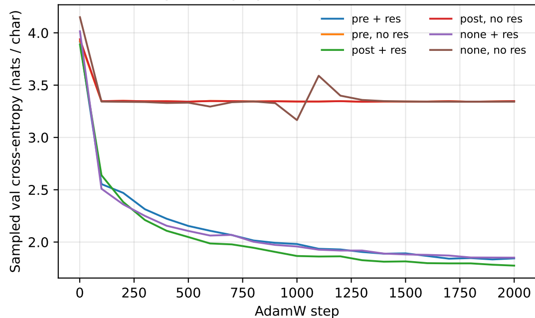
Training stability by norm placement x residual
