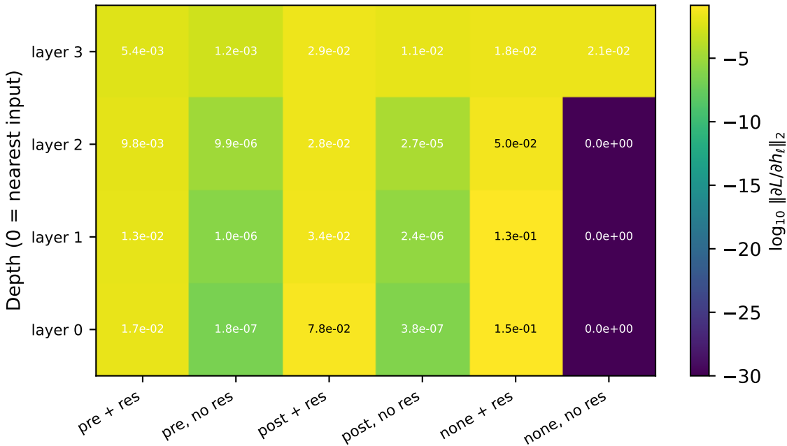
Per-layer gradient norm across norm/residual configs
