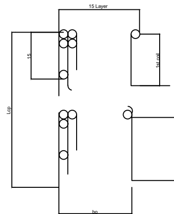
Fig 1.4 : Cross over Winding
