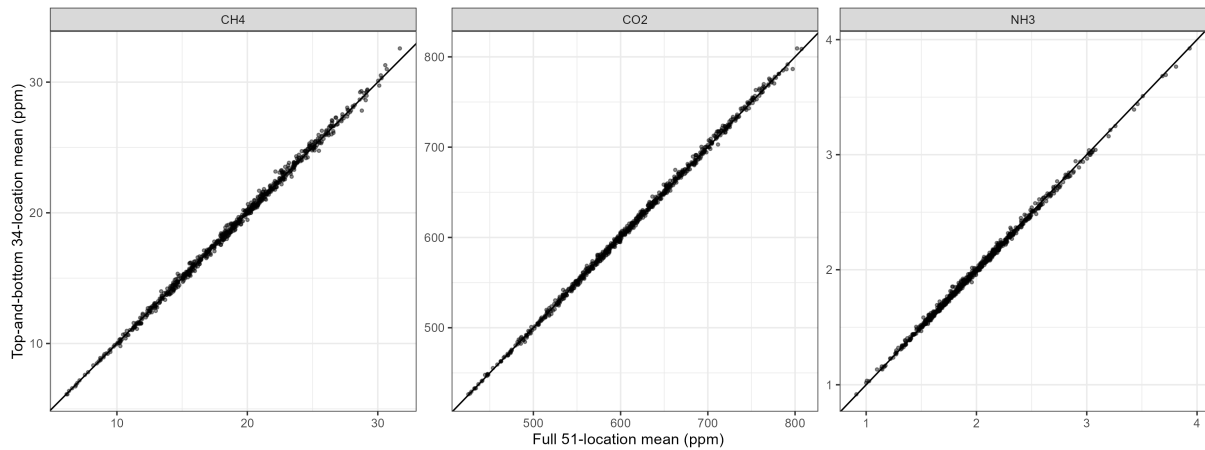
Figure 11: Agreement between the full 51-location mean and the reduced 34-location top-and-bottom mean in 743 complete two-hour blocks. Solid lines represent exact 1:1 agreement. CCC denotes Lin's concordance correlation coefficient, and bias is the mean relative difference from the full-density estimate.
