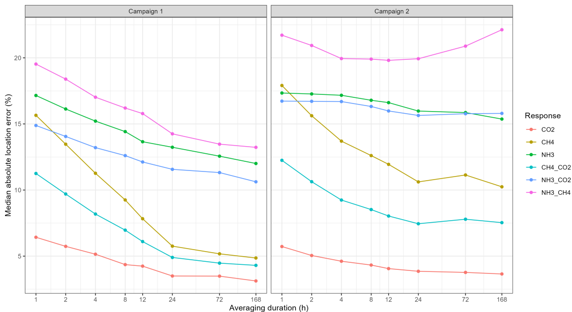
Figure 7: Convergence of median absolute location error as the averaging duration increased from 1 to 168 h. Errors were calculated relative to the contemporaneous measured-network mean. The logarithmic horizontal axis shows that concentration fields became more representative with aggregation but retained gas- and campaign-specific residual heterogeneity.
