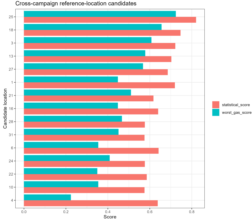
Figure 9: Leading cross-campaign reference-location candidates. The primary score equally combines concentration bias, absolute error, temporal stability, correlation, and mutual information after the physical exclusion criteria. The worst-gas score penalises candidates whose performance was poor for any one gas. Fan-corridor candidates were retained only in the sensitivity ranking.
