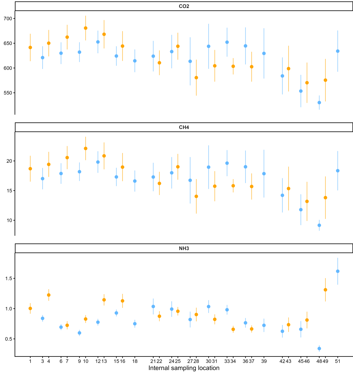
Figure 12: Campaign 2 concentrations measured with the reduced top-and-bottom network. Points denote means of daily location means and vertical bars denote 95% confidence intervals calculated across daily blocks. Orange and light-blue symbols denote top and bottom locations, respectively.
