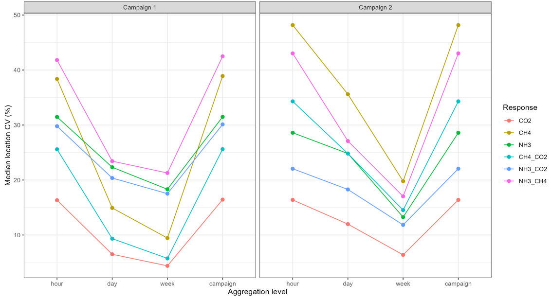
Figure 8: Median within-location coefficient of variation (CV) for CO 2 , CH 4 , NH 3 , and their three ratios at hourly, daily, weekly, and whole-campaign reporting scales. Hourly, daily, and weekly values quantify variability among block means, whereas the whole-campaign value was calculated directly from every valid observation and therefore preserves the full seasonal and diurnal range. Consequently, the whole-campaign bar should not be interpreted as a continuation of the temporal averaging sequence.
