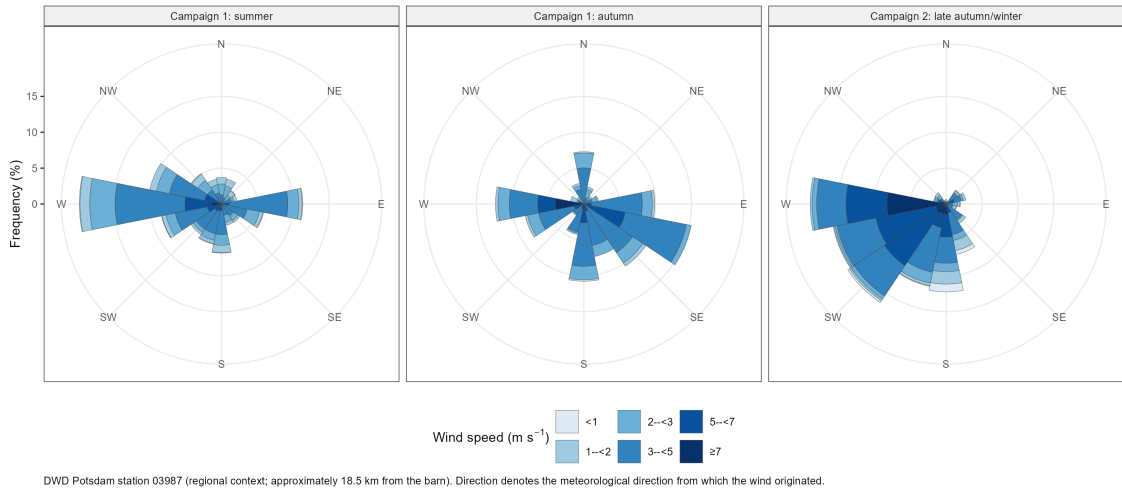
Figure 5: Wind roses for the three experimental periods constructed from hourly DWD Potsdam station 03987 observations. Colours show wind-speed classes and radial length shows the percentage of valid hourly observations in each directional sector. Direction denotes the meteorological direction from which the wind originated. The station is approximately 18.5 km from the barn; the figure therefore describes regional conditions rather than barn-local airflow.
