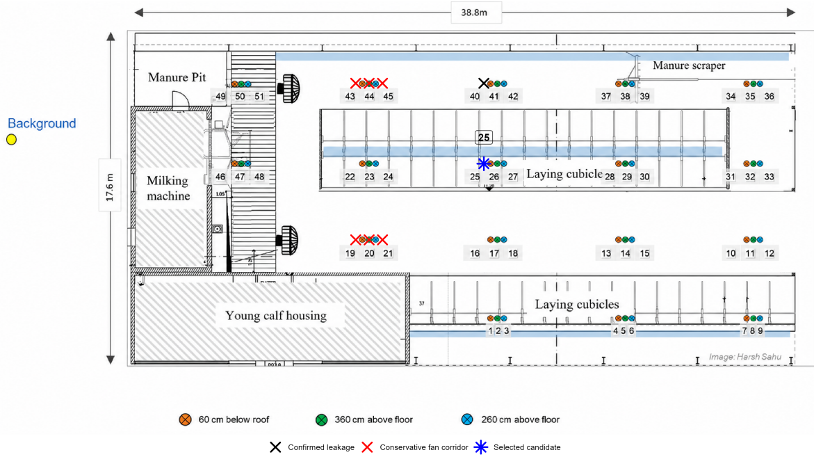
Figure 10: Physical screening of the statistically selected reference candidate. Location 25 is marked in blue. Red crosses identify the conservatively excluded fan corridors containing locations 19–21 and 43–45; the black cross marks location 40, which was excluded because of confirmed sampling-line leakage. The exact fan axes should be confirmed against the operational installation before final engineering acceptance.
