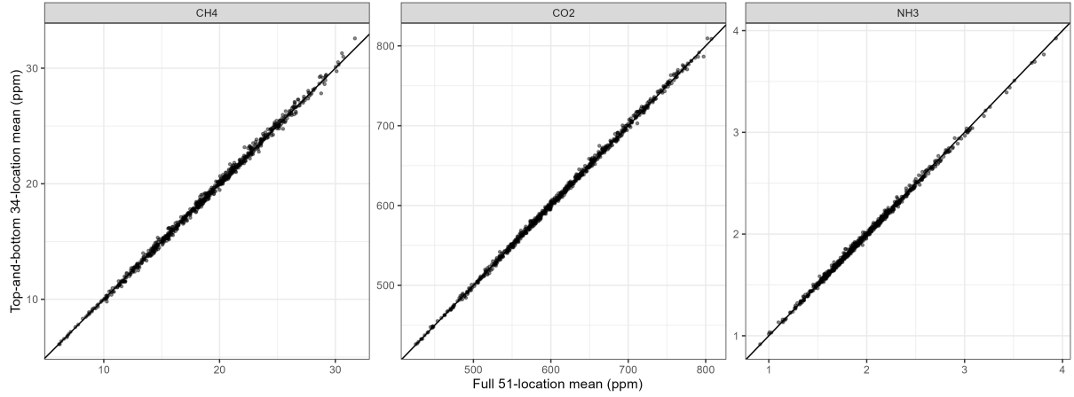
Figure 12: Agreement between the full 51-location mean and the reduced 34-location top-and-bottom mean in 743 complete two-hour blocks. Solid lines represent exact 1:1 agreement. CCC denotes Lin’s concordance correlation coefficient, and bias is the mean relative difference from the full-density estimate.
