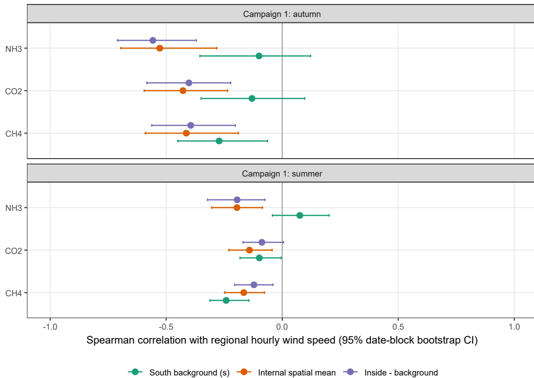
Figure 7: Exploratory contemporaneous associations between regional hourly DWD wind speed and three Campaign 1 concentration outcomes: the south-background location s , the internal spatial mean, and the internal-minus-background enhancement. Points are Spearman correlations and horizontal bars are 95% confidence intervals obtained by re-sampling complete dates. Summer and autumn were analysed separately. DWD wind speed describes regional conditions and is not a measurement of barn-local wind or turbulence intensity.
