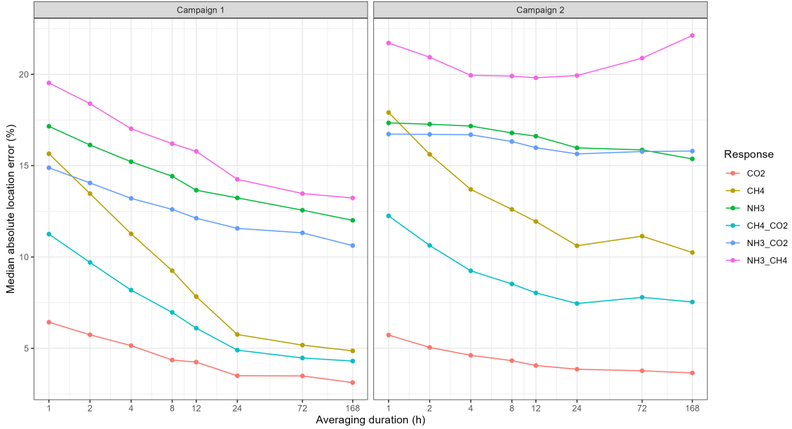
Figure 8: Convergence of median absolute location error as the averaging duration increased from 1 to 168 h. Errors were calculated relative to the contemporaneous measured-network mean. The logarithmic horizontal axis shows that concentration fields became more representative with aggregation but retained gas- and campaign-specific residual heterogeneity.
