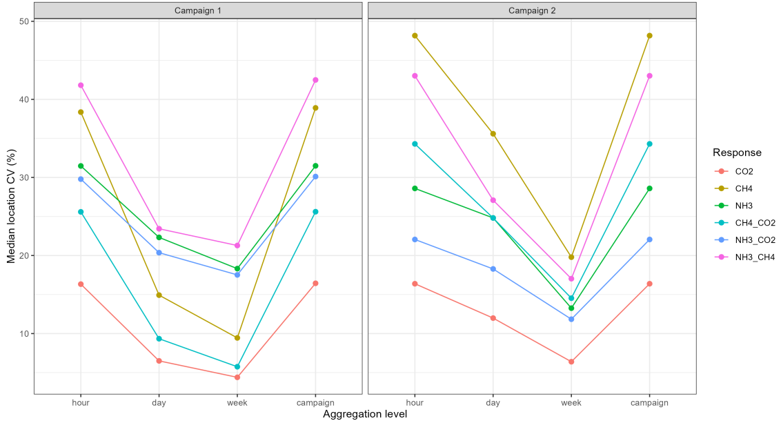
Figure 9: Median within-location coefficient of variation (CV) for CO 2 , CH 4 , NH 3 , and their three ratios at hourly, daily, weekly, and whole-campaign reporting scales. Hourly, daily, and weekly values quantify variability among block means, whereas the whole-campaign value was calculated directly from every valid observation and therefore preserves the full seasonal and diurnal range. Consequently, the whole-campaign bar should not be interpreted as a continuation of the temporal averaging sequence.
