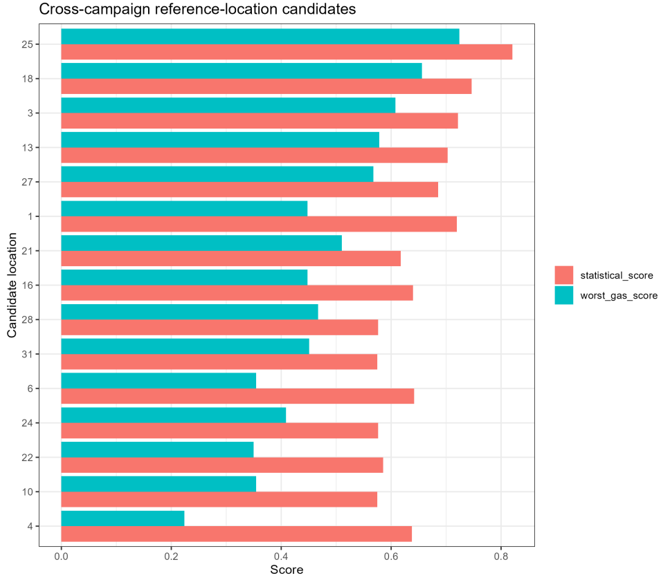
Figure 10: Leading cross-campaign reference-location candidates. The primary score equally combines concentration bias, absolute error, temporal stability, correlation, and mutual information after the physical exclusion criteria. The worst-gas score penalises candidates whose performance was poor for any one gas. Fan-corridor candidates were retained only in the sensitivity ranking.
