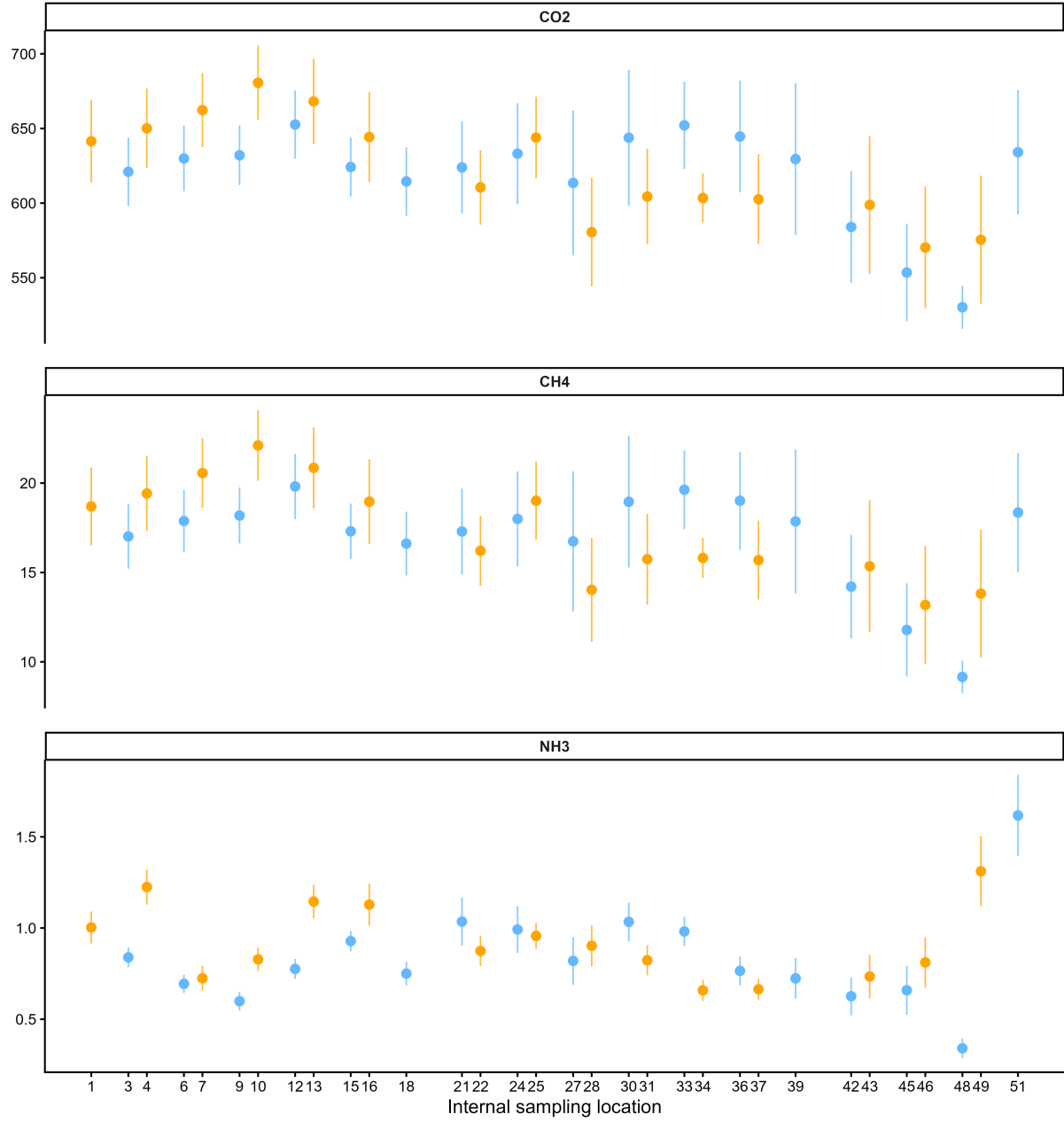
Figure 13: Campaign 2 concentrations measured with the reduced top-and-bottom network. Points denote means of daily location means and vertical bars denote 95% confidence intervals calculated across daily blocks. Orange and light-blue symbols denote top and bottom locations, respectively.
