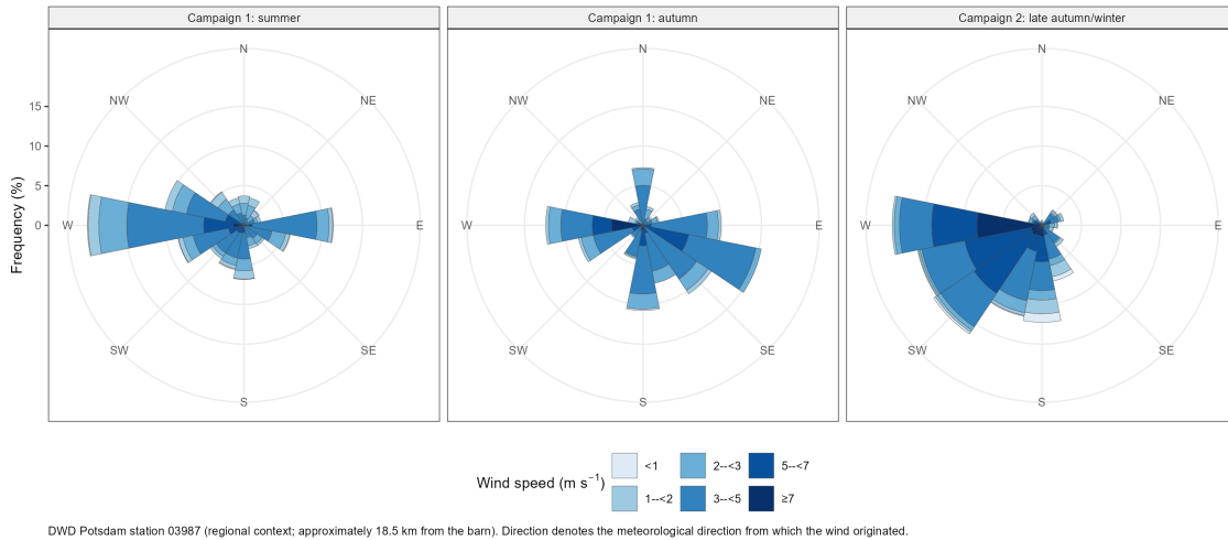
Figure 5: Wind roses for the three experimental periods constructed from hourly DWD Potsdam station 03987 observations. Colours show wind-speed classes and radial length shows the percentage of valid hourly observations in each directional sector. Direction denotes the meteorological direction from which the wind originated. The station is approximately 18.5 km from the barn; the figure therefore describes regional conditions rather than barn-local airflow.
