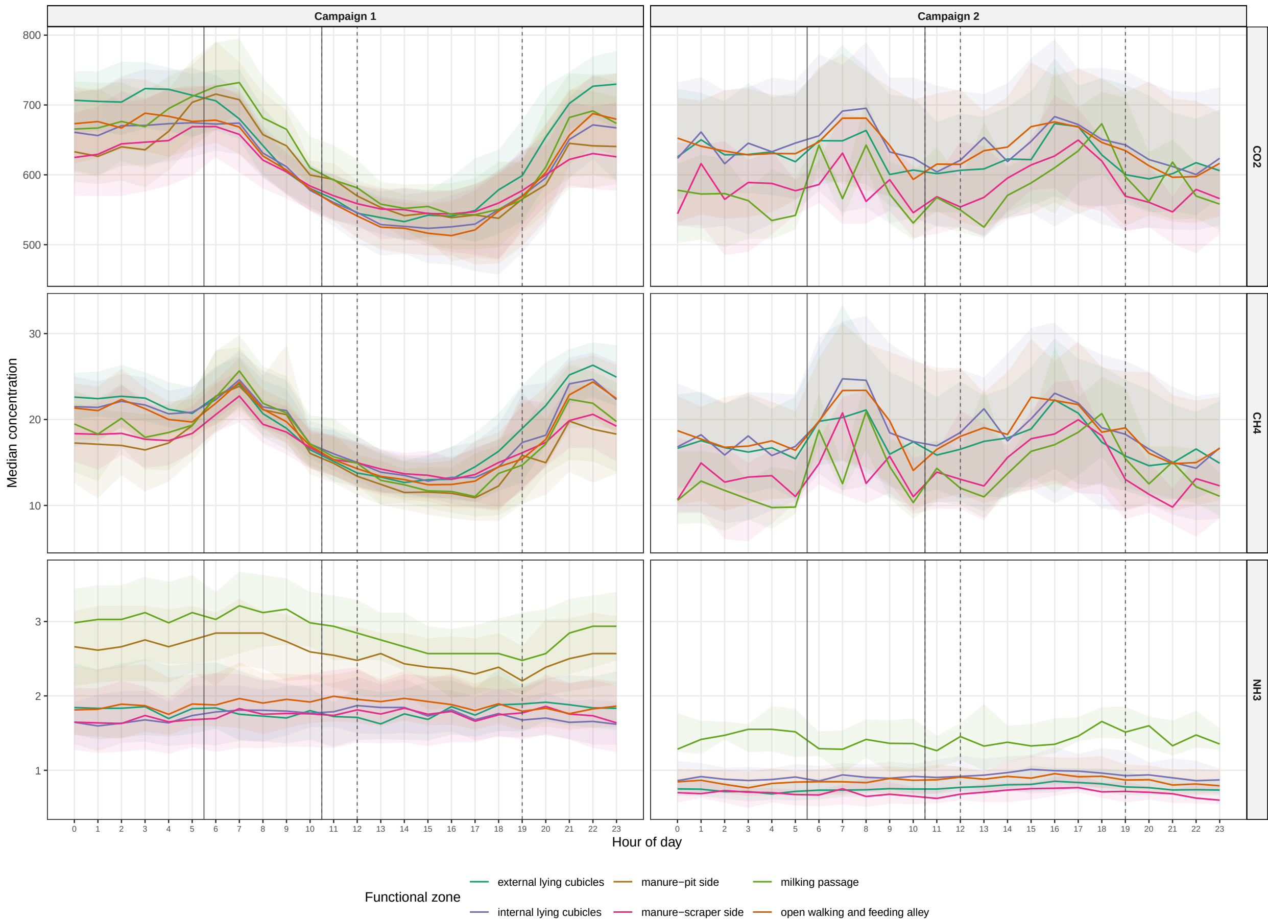
Diurnal concentration profiles by functional barn zone Solid lines: feeding at 05:30 and 10:30; dashed lines: feed pushing at 10:30, 12:00 and 19:00
