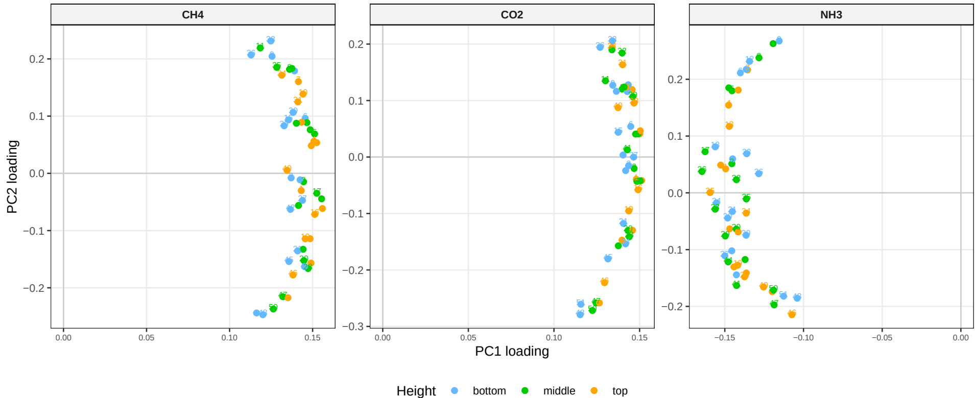
Campaign 1 PCA loadings by sampling height
