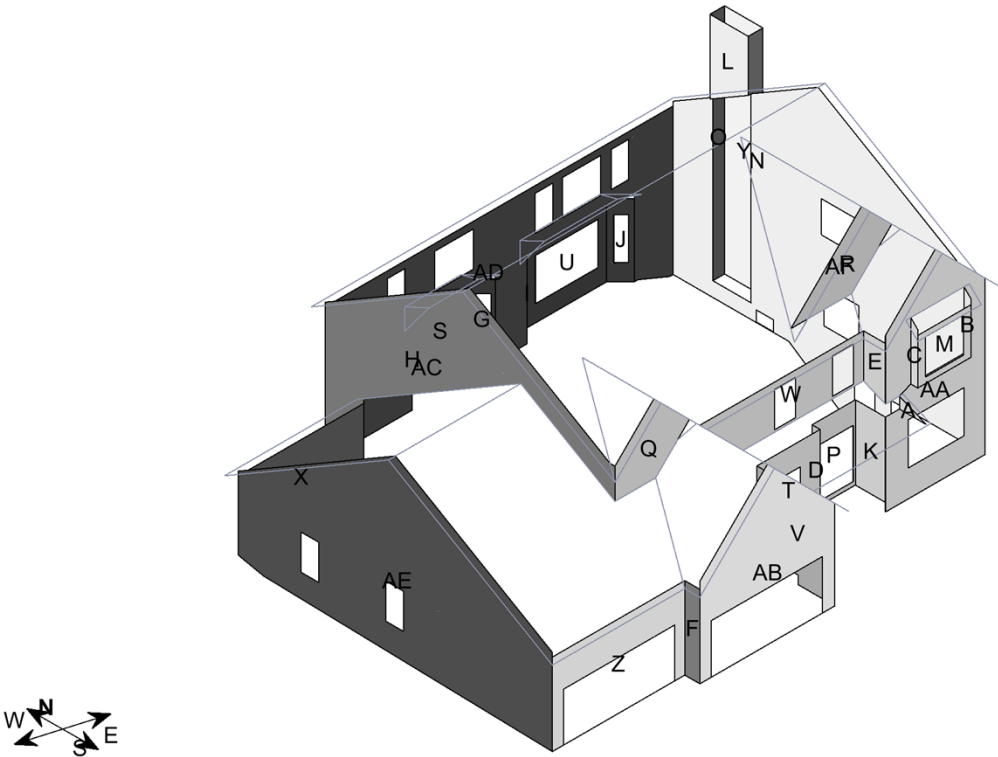
Wall Area by Direction
